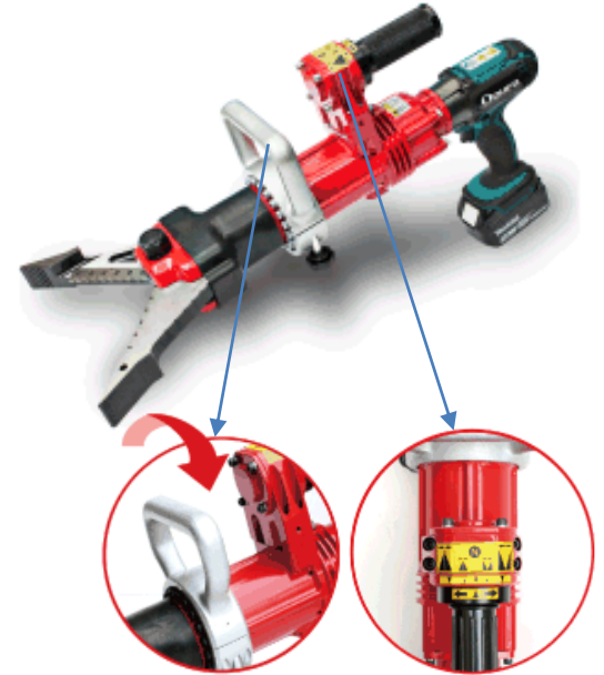
HRS-931 Pump-unit
